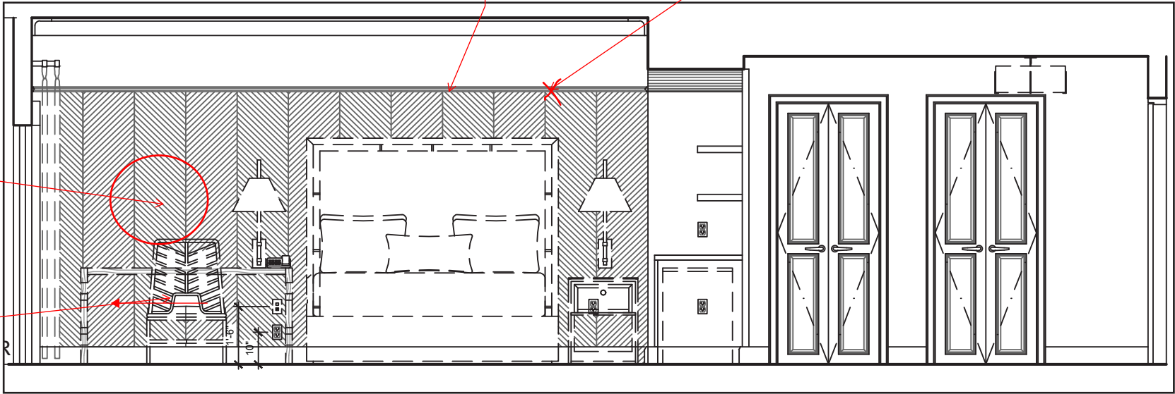
ELEVATION 02 NTS
