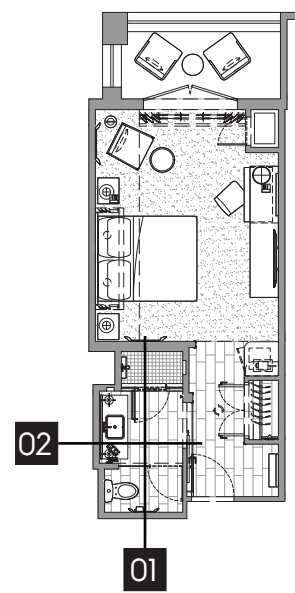
FLOOR PLAN
